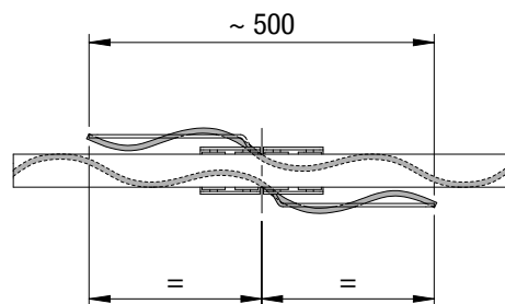
OVERLAP DIMENSIONS
