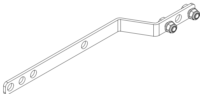
1T14 Overlap Arms Kit (2 pcs)
