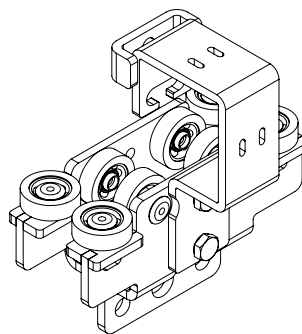
1T12 Master Carrier Top Cord System
