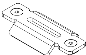
1T04 Overlap Bridge
