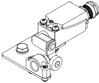
1T50 Limit Switch Side Cord System
