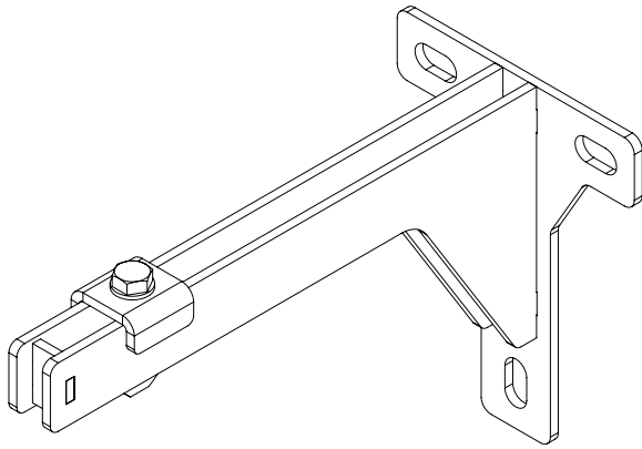
1Z10-250 Wall Bracket 250mm
