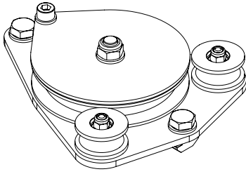
1T20 Return Pulley
