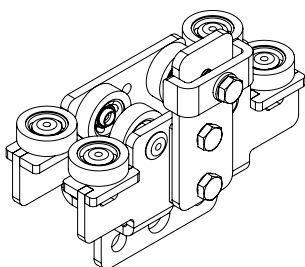
1T11 Master Carrier Side Cord System
