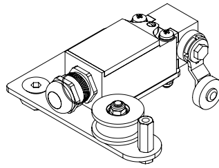
1T52 Limit Switch c/w Pulley Top Cord System
