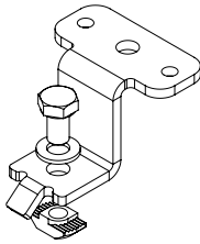
1T30 Suspension Bracket for Side Cord System
